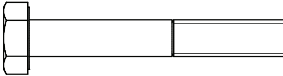
PART # 49 HEX HEAD BOLT M10X70L PARTIAL THREAD QTY.5
