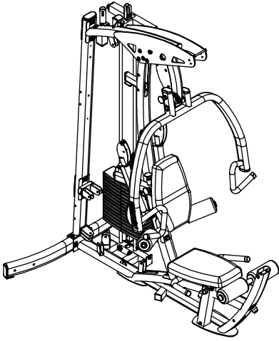
Above shows STEP 6 assembled and completed
