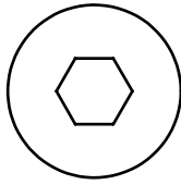
PART# 08 ALLEN HEAD BOLT M12X20L FULL THREAD QTY.2
