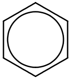
PART # 56 HEX HEAD BOLT M10X90L PARTIAL THREAD QTY.1
