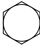
PART # 51 HEX HEAD BOLT M10X50L PARTIAL THREAD QTY.1
