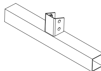
PART C LEFT LOWER FRAME [1 PCS]
