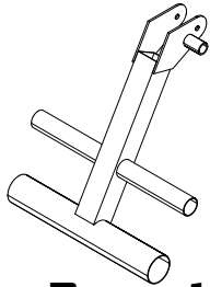
PART 1 FOLDING LEG [1 PCS]
