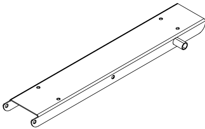
PART 4 BACK PAD FRAME [1 PCS]
