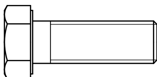
Part #10 HEX HEAD BOLT M10X25mm
