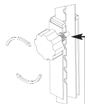
Shows pop pin plunger is fully engaged.
