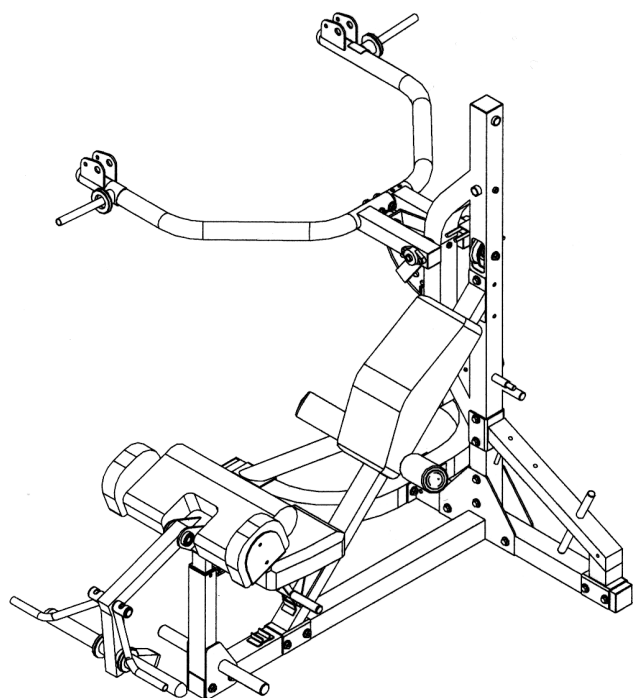
Above shows STEP 8 assembled and completed.
