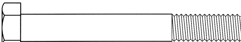
Key # (33) hex bolt 12mm x 95mm partial thread QTY. 1
