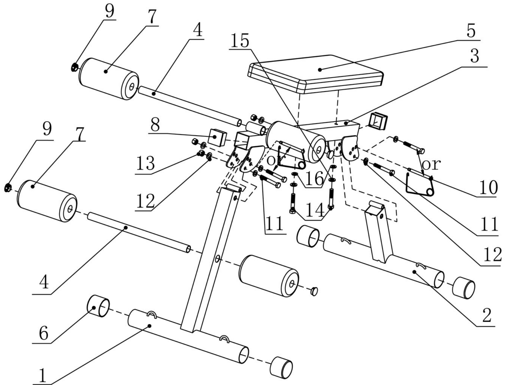
BFAB10 Exploded View
